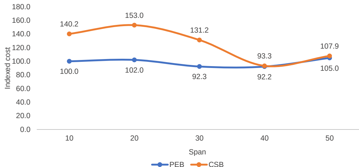
Cost of per square metre of pre-engineered building and conventional steel structure
